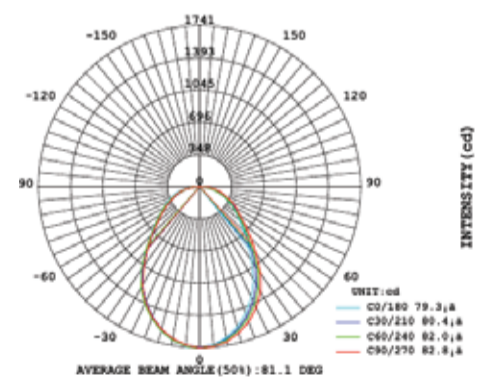
LUMINOUS INTENSITY DISTRIBUTION
